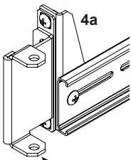
Short CMA Bracket Attached to Rack using Rack mount screws
