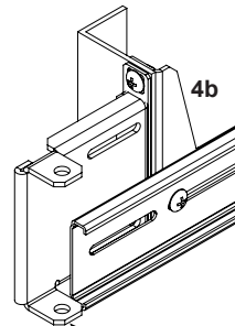
CMA Bracket Attached to Rack using Rack mount screws
