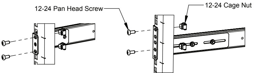
Rear Rack Attachment
