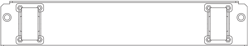
Fixed Caster Plate – This Side Installed at Rear of Rack
