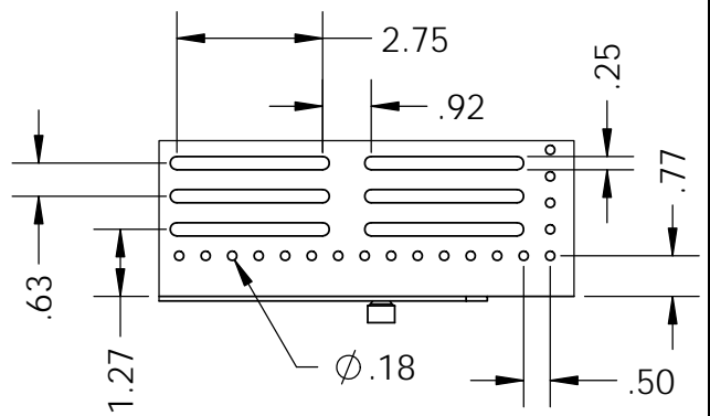
DETAIL A SLOTTED HOLE DIMENSION ALL DIMENSIONS TYPICAL
