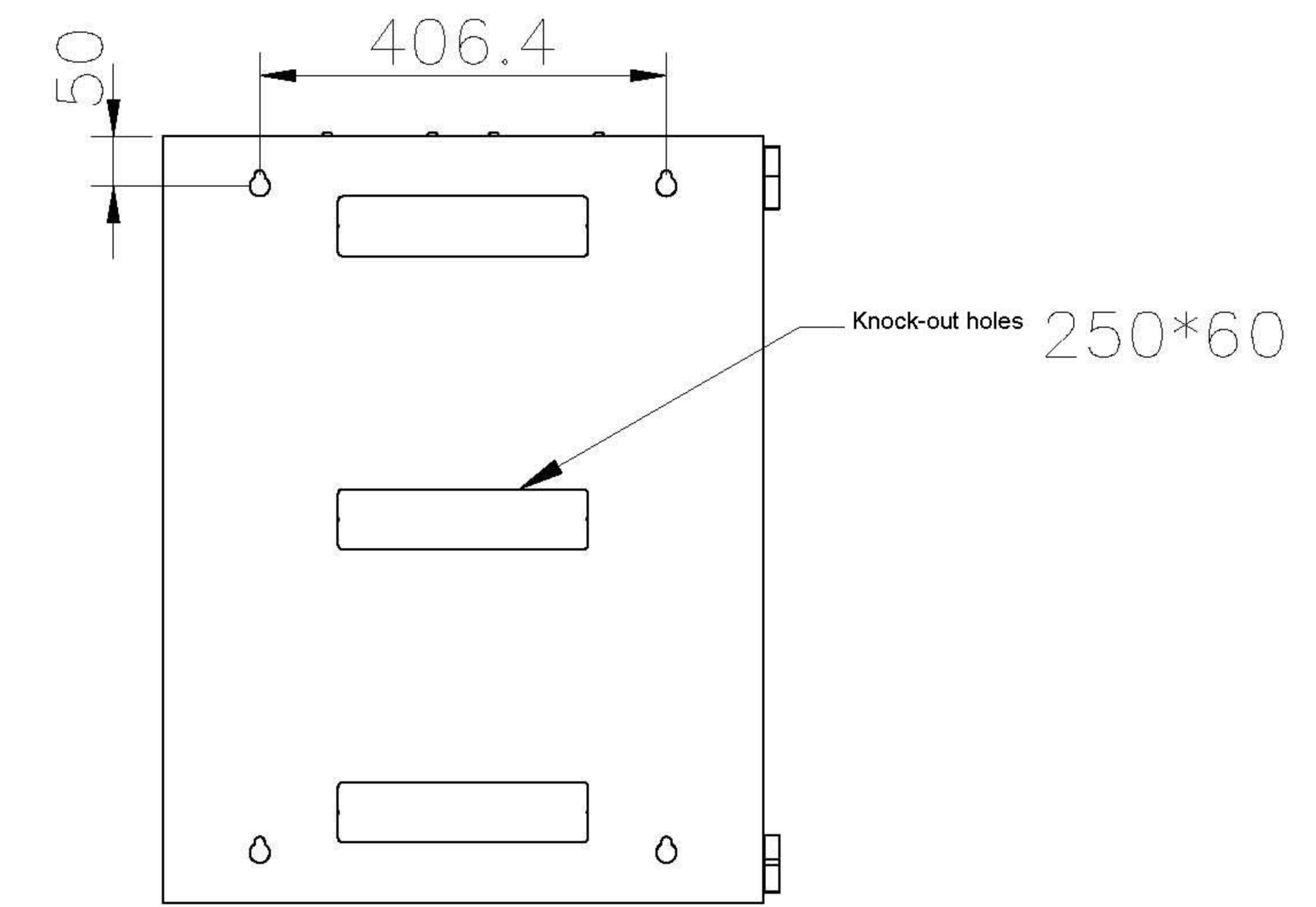
Back view for cabinet
