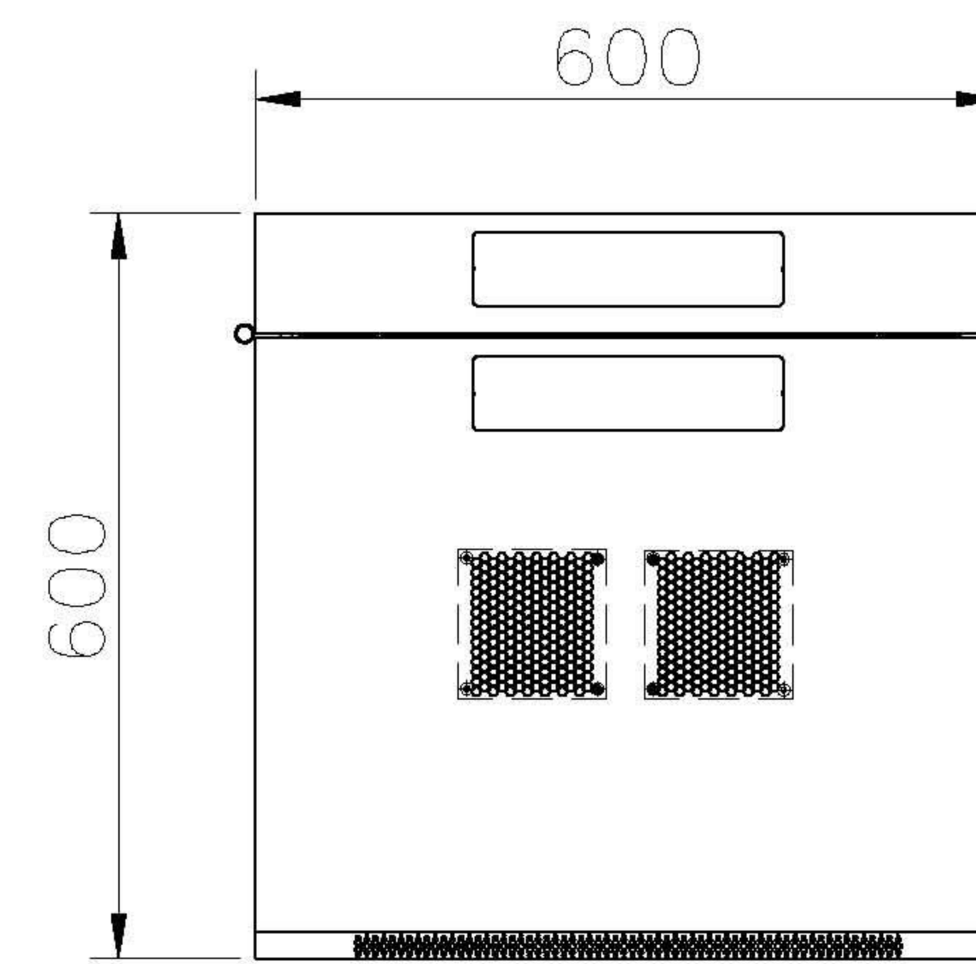
Up view for cabinet
