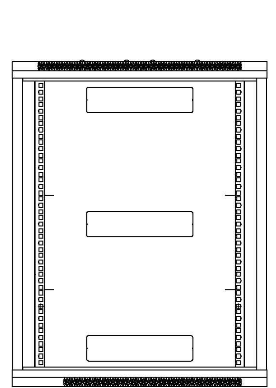
Front view for cabinet(without front door)
