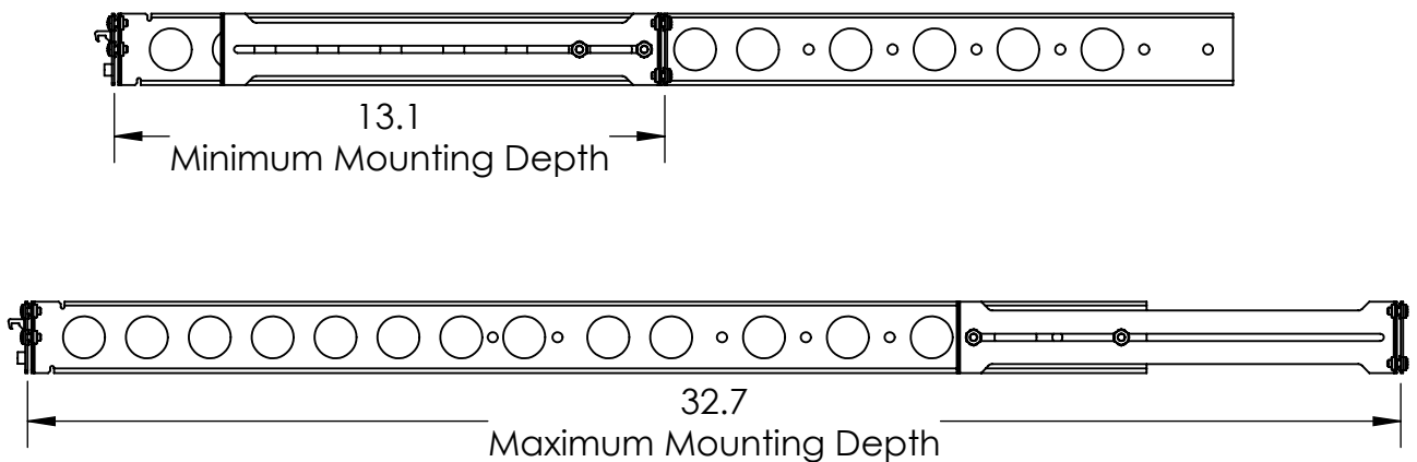
Outer Rail Exterior View
