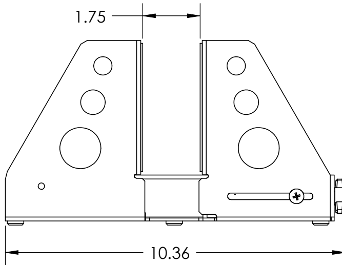
1U Configuration
