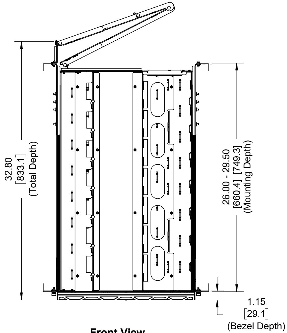
Front View
