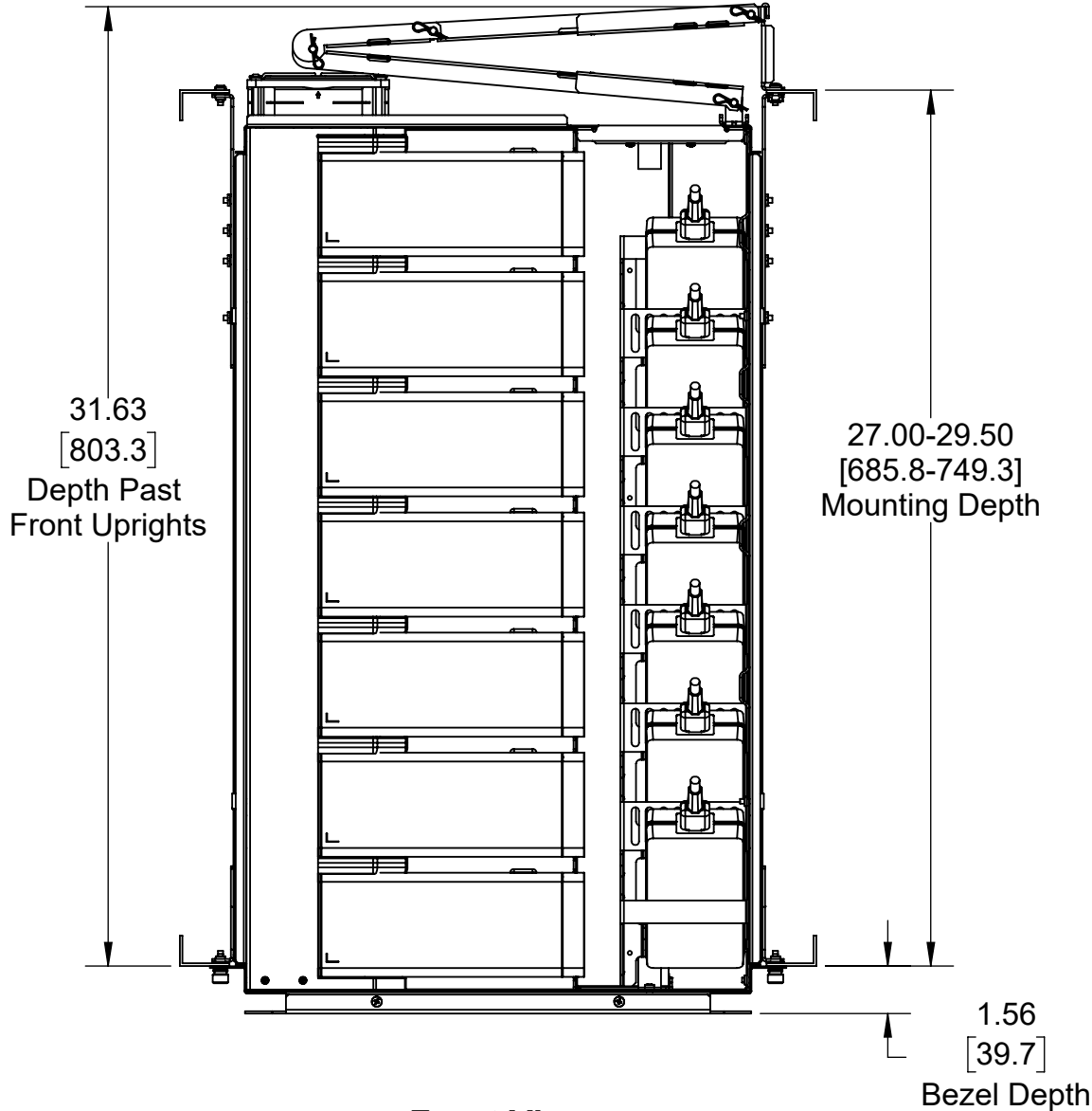
Front View
